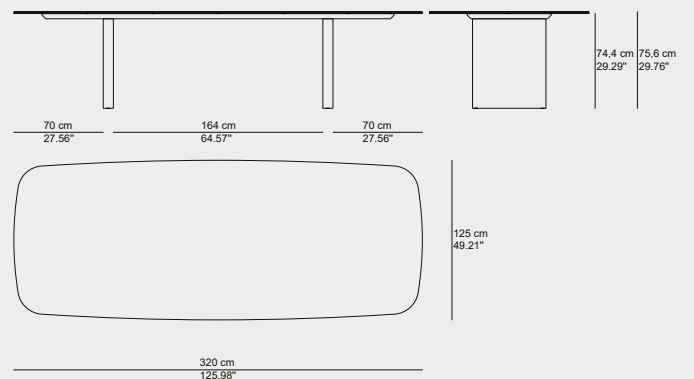
DINING TABLE - 320X125CM 03254-XX-XX
